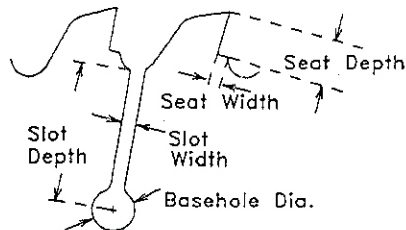
"STD." Standard Slot Slot with Open Basehole
